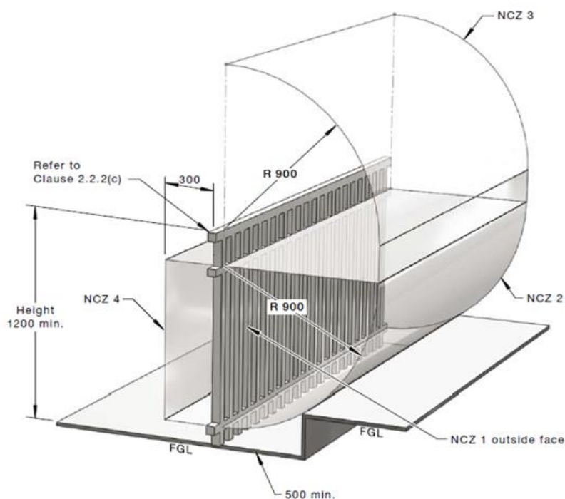
Figure 1 - Example of Non-Climbable Zones, referenced from AS1926.1, Figure 2.1
